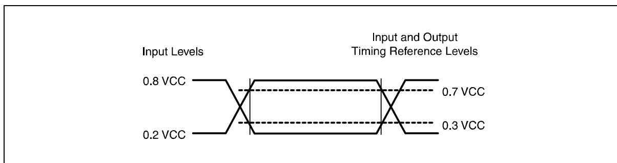
Figure 23. AC Measurement I/O Waveform
